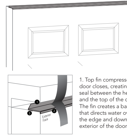
7/8" Top seal application
