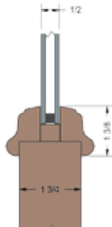
Raised Molding 1/2" I.G.
