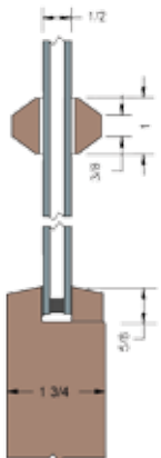
Tapered Mission Molding & 1" SDL Bar
