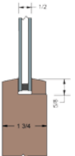
Tapered Mission Molding 1/2" I.G.
