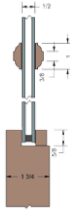
Mission Molding & 1" SDL Bar
