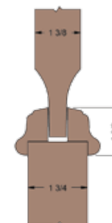
Raised Panel Molding Standard Panel
