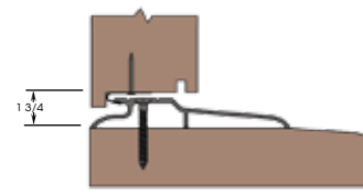
Interlocking Sill
