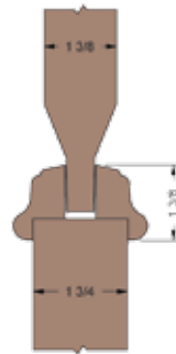
Raised Panel Molding Traditional Panel
