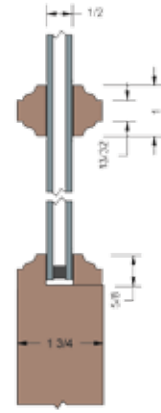
Recessed Molding Style C & 1" SDL Bar
