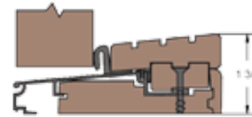
Impact Bumper Sill B
